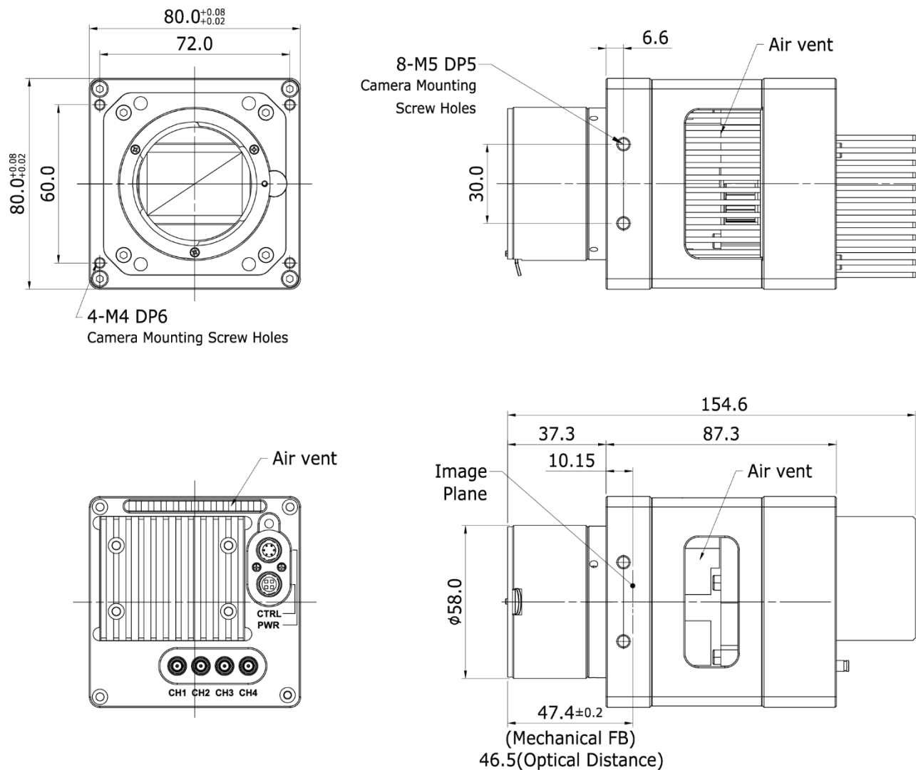
Figure 5.4 Mechanical Dimension for VP-61MX-18 H F-mount
