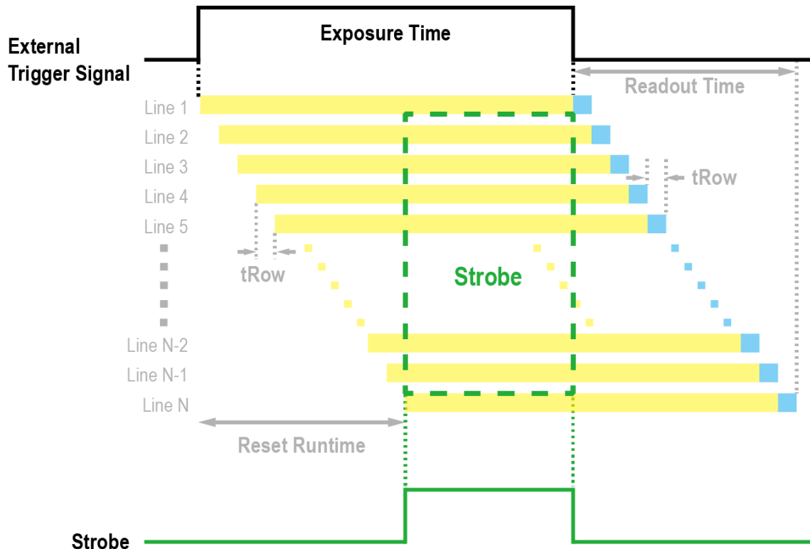
Figure 9.11 Strobe Signal
