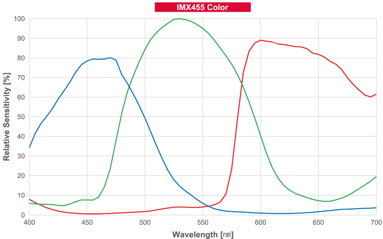
Figure 5.3 VP-61MX-C18 H Spectral Response
