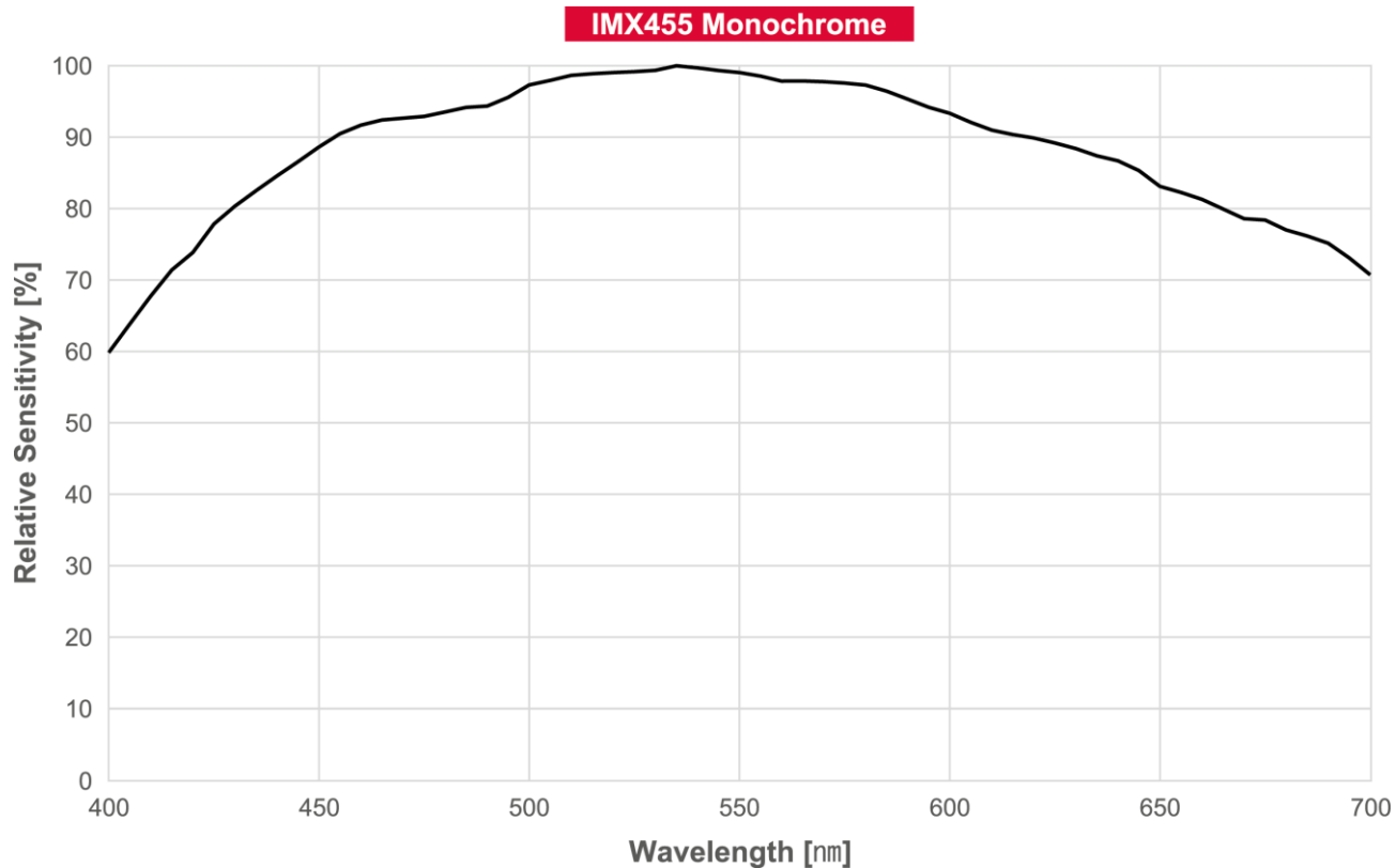
Figure 5.2 VP-61MX-M18 H Spectral Response
