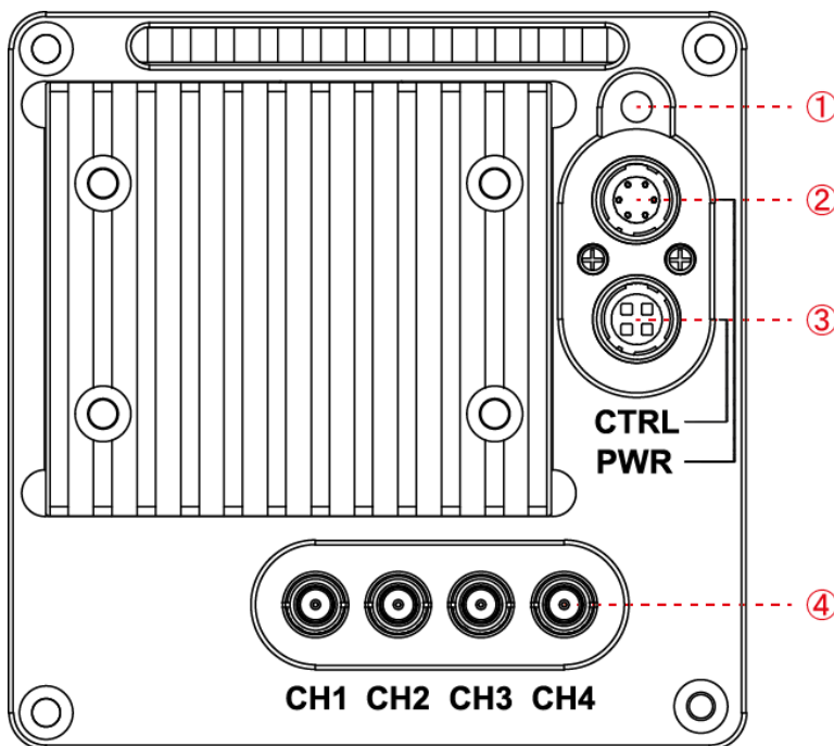
Figure 7.1 VP-61MX-18 H with DIN 1.0/2.3-type Connectors
